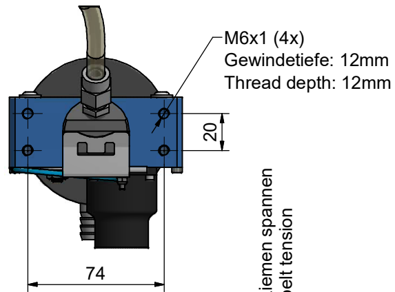
View B ( 1 : 2 )
